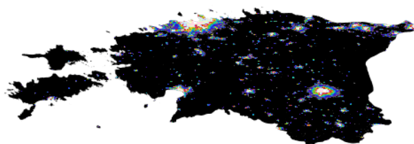
Fig. 16: Estonia's sky brightness
