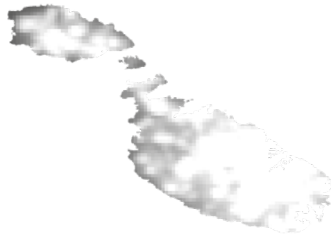
Fig. 43: Malta's night lights
